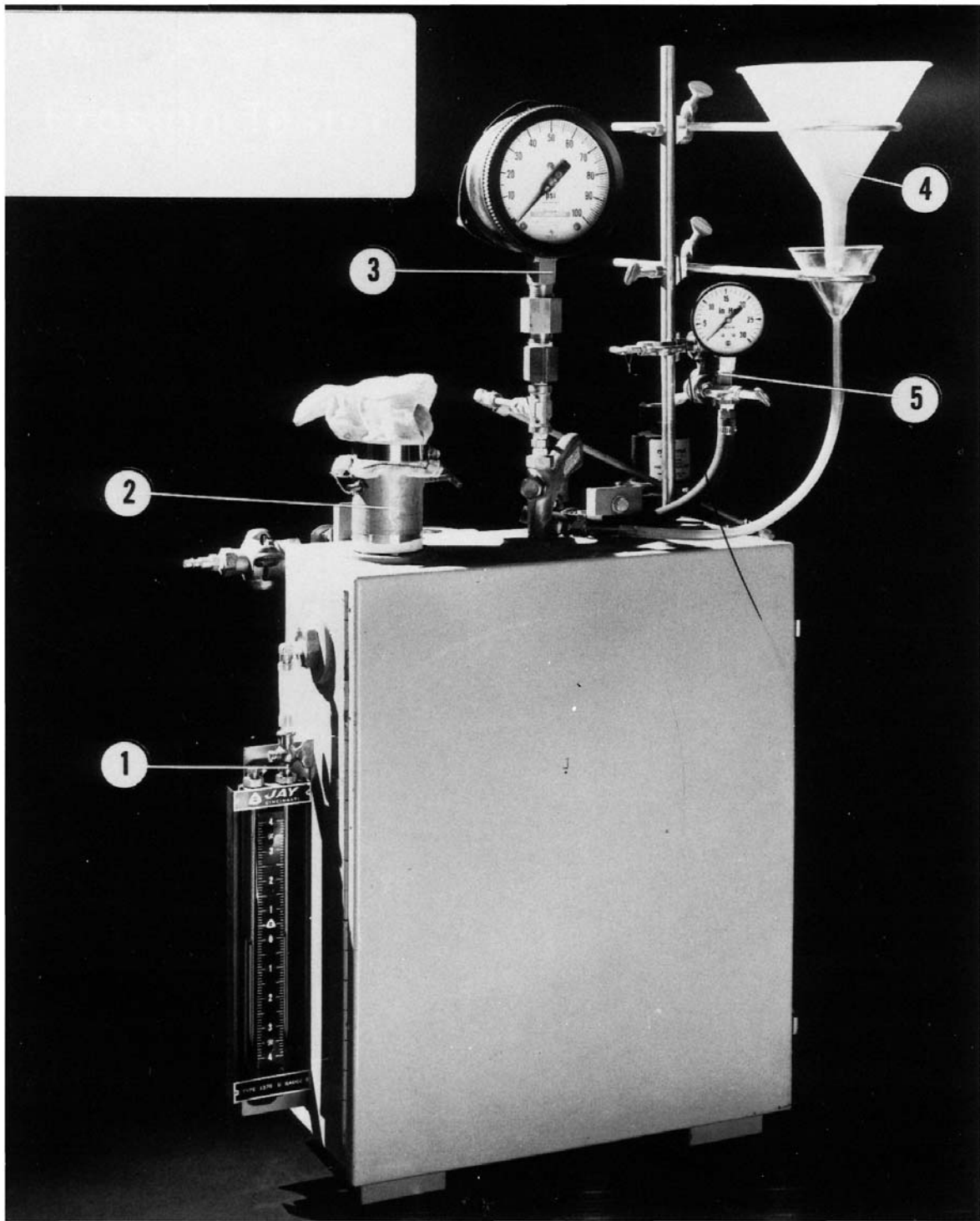
FIG. 1 Abrasion Tester
